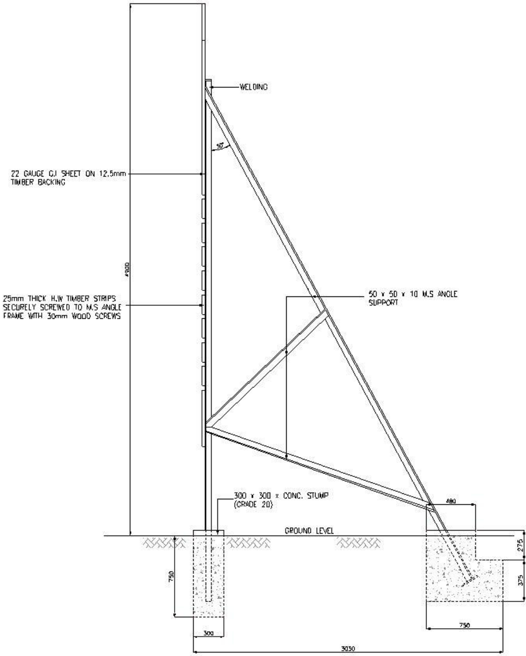
SIDE VIEW
