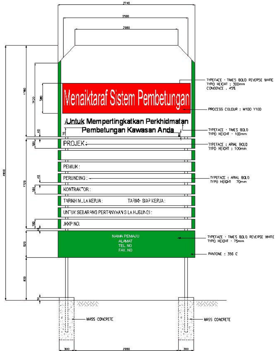
FRONT VIEW
